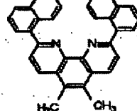
Structural formula 10:
